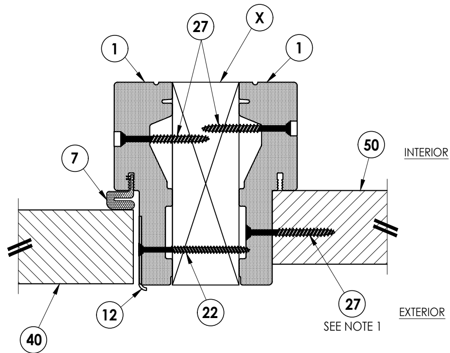
2 5 HORIZONTAL CROSS SECTION
