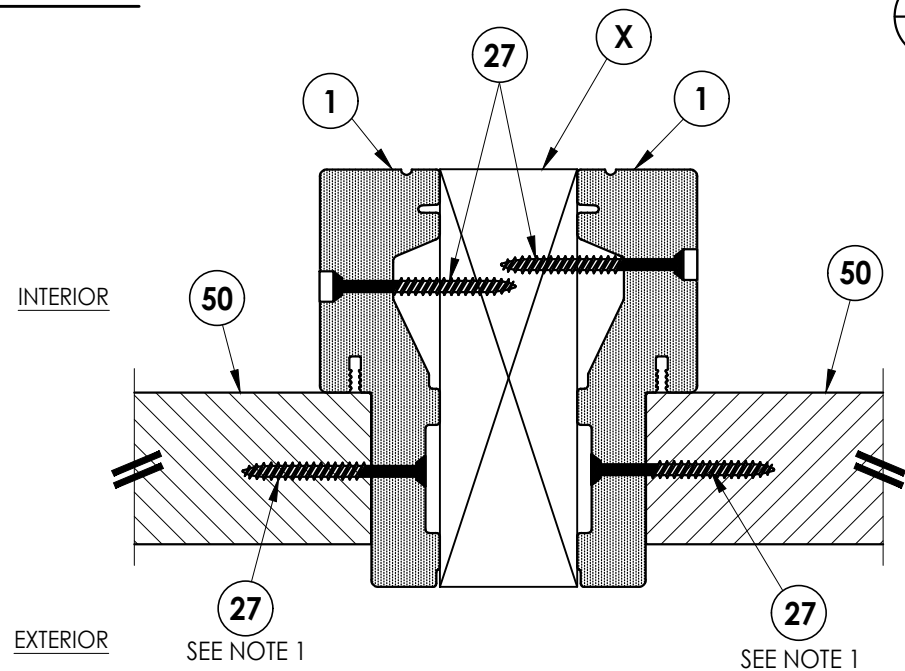
3 5 HORIZONTAL CROSS SECTION
