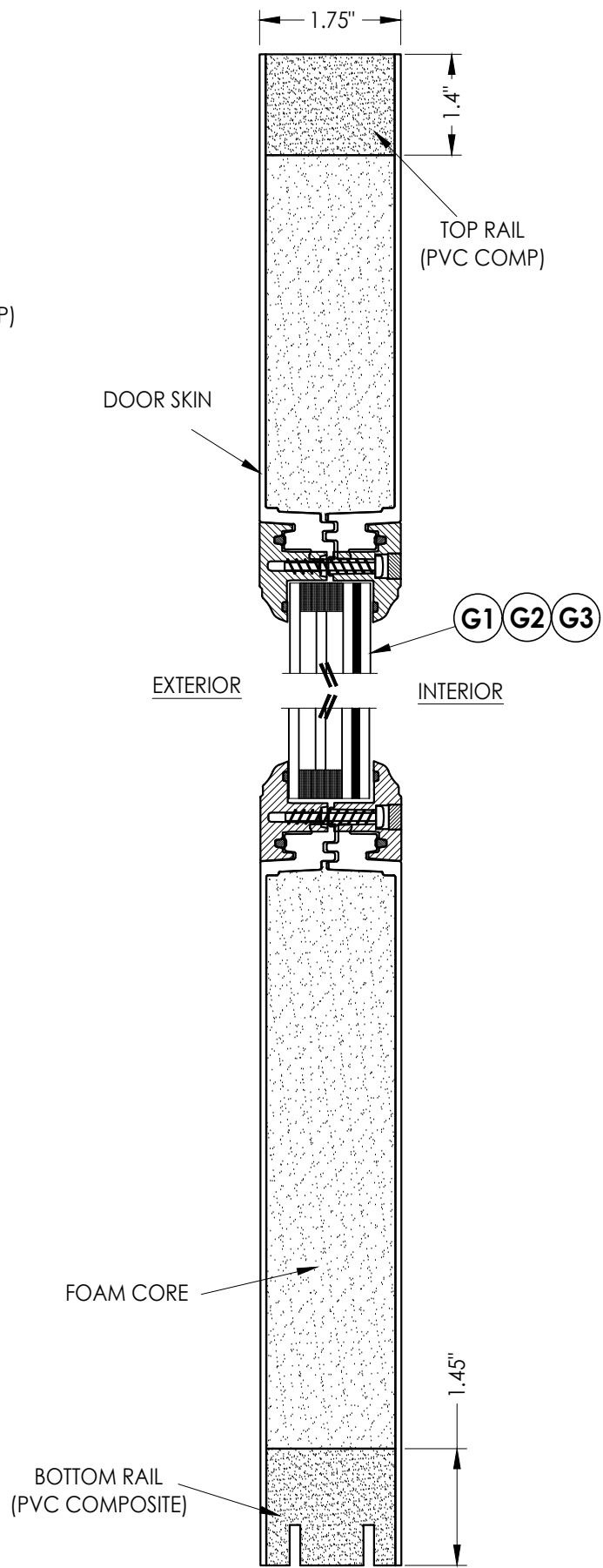
2 2 VERTICAL CROSS SECTION
